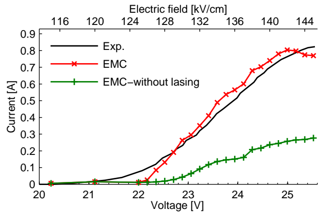
FIG. 1. (Color online) Current-voltage characteristics. The EMC simulation results with (X marks) and without (crosses) lasing included are compared to available experimental data 3 (solid curve). The electric current is governed by stimulated photon emission and absorption processes, as has to be expected for a WPE as high as 50%.
