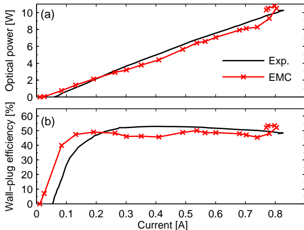
FIG. 2. (Color online) (a) Current-optical power and (b) current-WPE characteristics. The EMC simulation results with lasing included (X marks) are compared to available experimental data 3 (solid curve).
