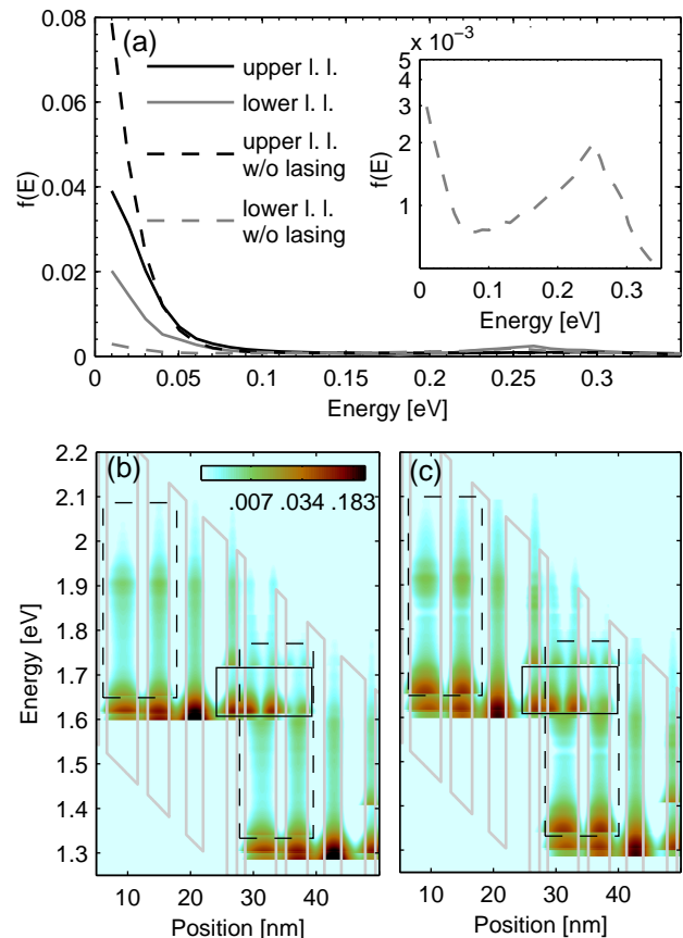
FIG. 3. (Color online) (a) Simulated kinetic electron distribution f(E) in the upper and lower laser level with and without lasing included. (b) Energy resolved electron density without lasing included; (c) energy resolved electron density with lasing included. The upper laser levels are marked by solid rectangles, and the lower laser level is marked by dashed rectangles.
